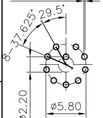
PCB Layout
