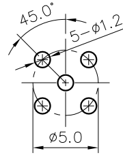
PCB Layout
